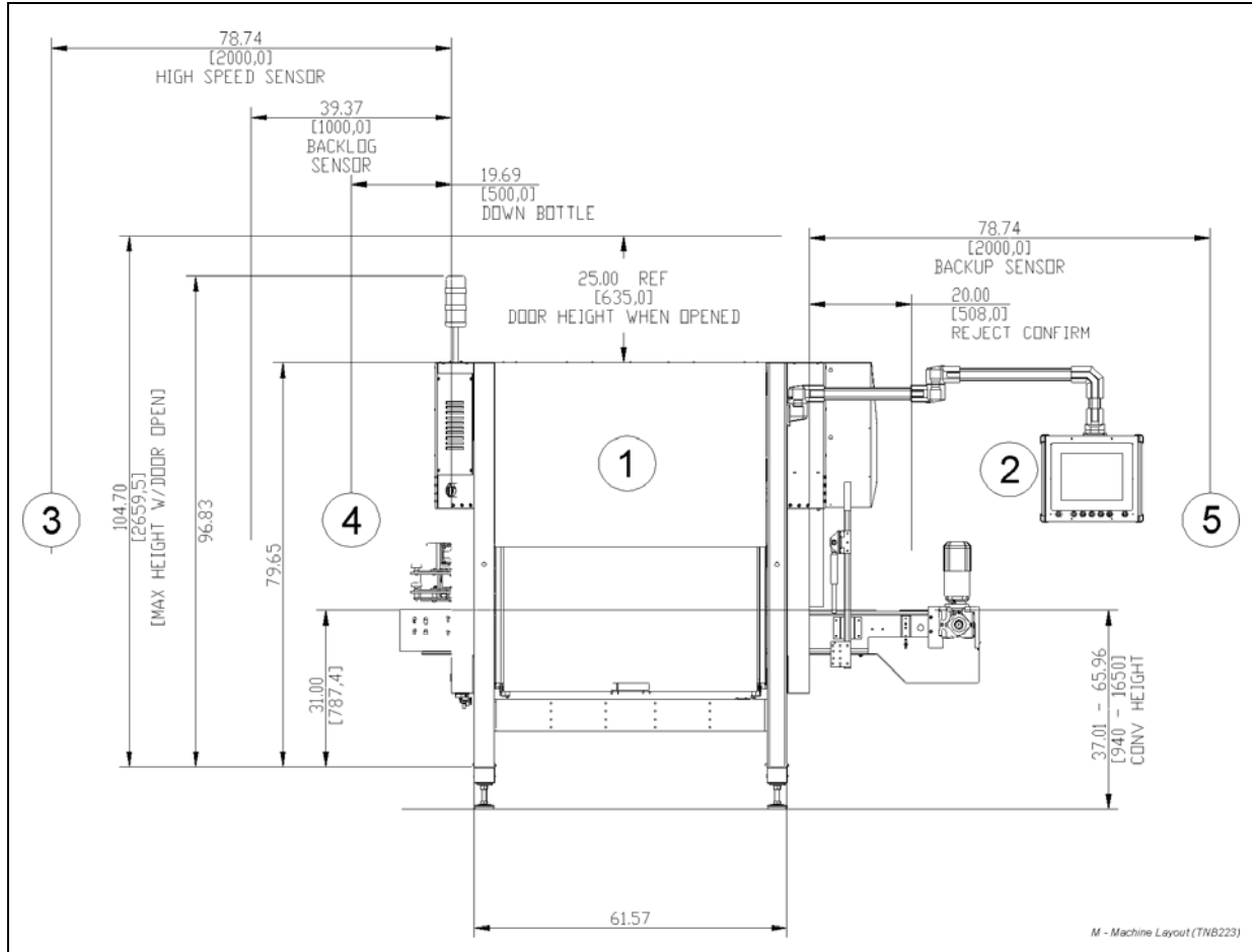
FleX M Machine Layout Drawing (ref. 9016C25)
